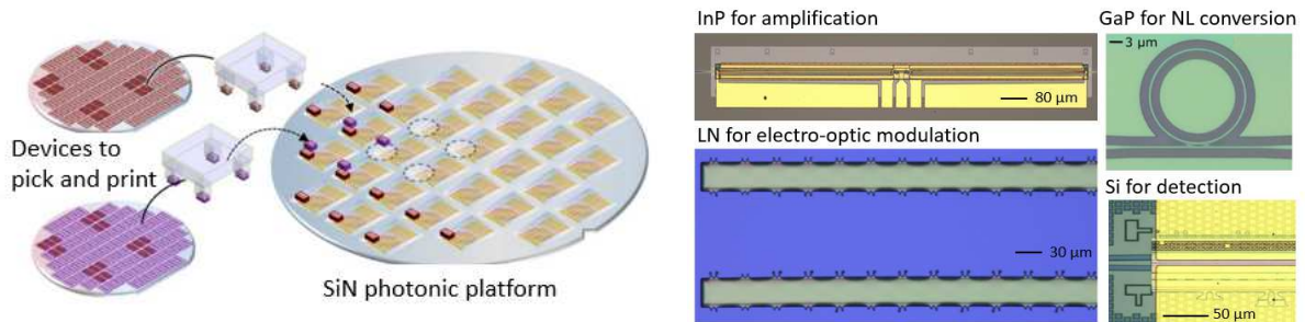
Figure - 1) Illustration of devices hetero-integration on a SiN wafer via micro-transfer printing and microscope pictures of transfer printed devices
